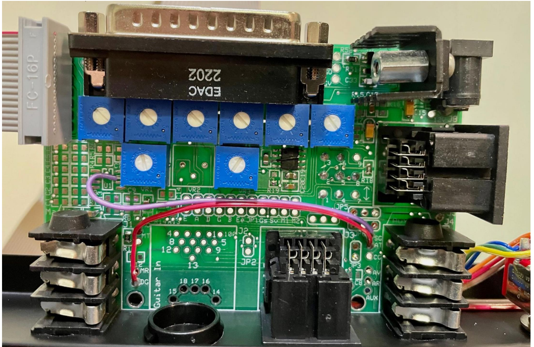
AMB-13P-2 (Roland BC-13 Replacement) Semi-Populated PC Board that is mounted to the Break-Out-Rack via the Mag & Aux 1/4" Connectors
